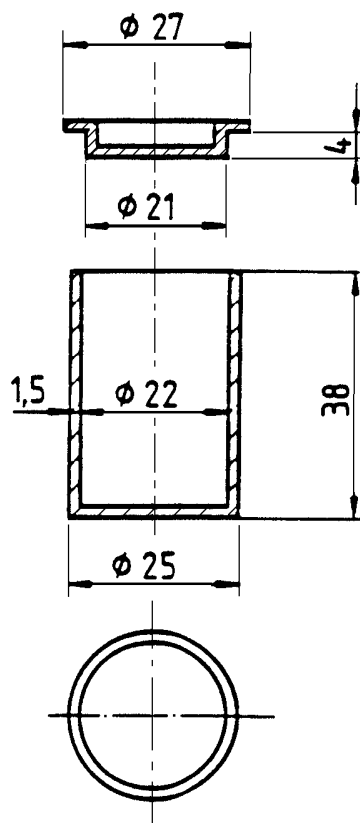
Figure 1 — Silica crucible and lid crucible made of silica must be used.
